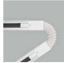
4010 Flexible connector To connect two track sections at any angle up to 90° or wall to ceiling or pitched ceiling applications.
