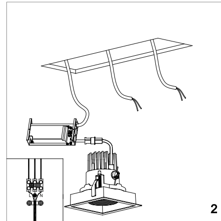
2 Place the mounting frame into the hole of the ceiling;
