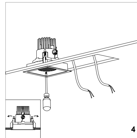
4 Paint around the mounting hole to make the ceiling have a flat appearance;
