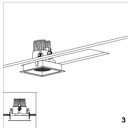
3 Fix the mounting frame in the ceiling with screws;
